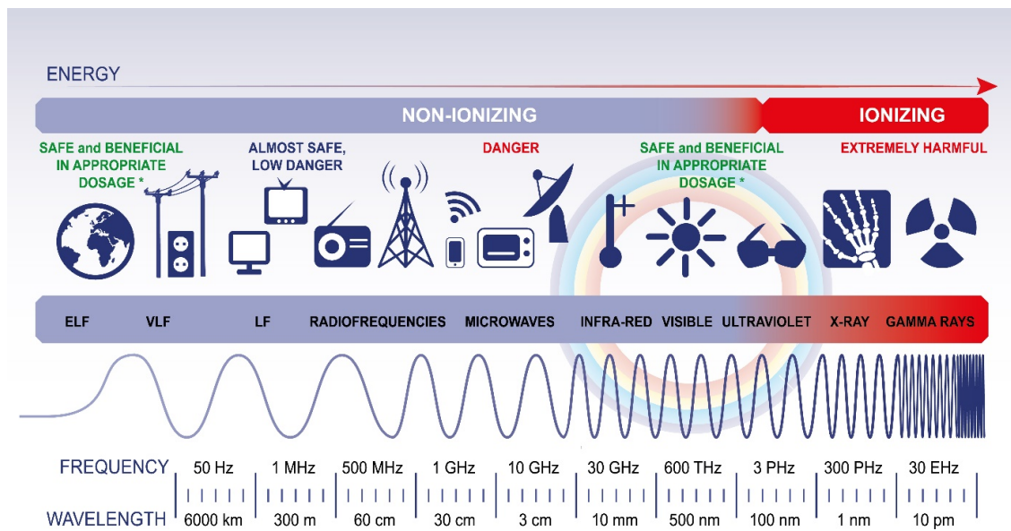
Figure 1 – Electromagnetic spectrum
